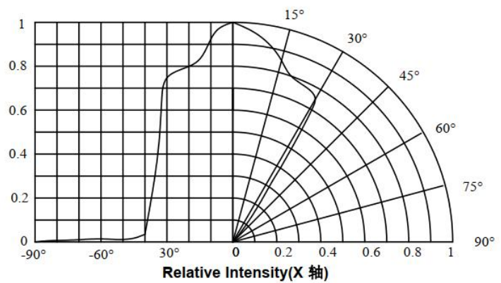
Fig.6 Radiation Diagram
