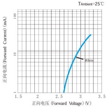
伏安特性 Volt-Ampere Characteristics
