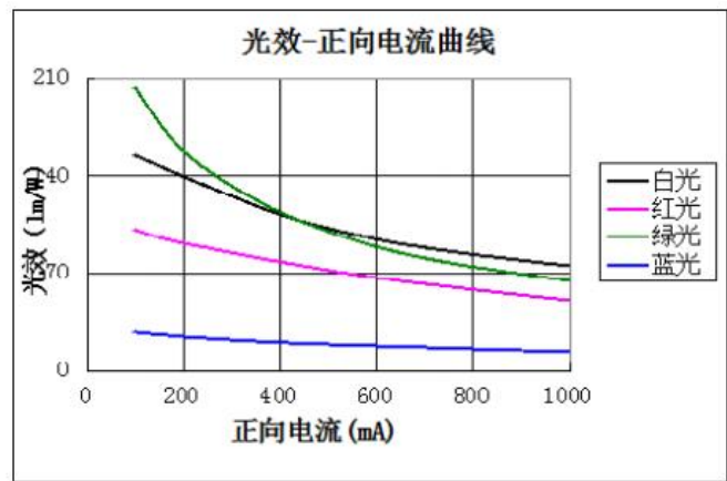
Fig 3. IF-Lm/W, T_a = 25^\circ\text{C} , RH60%
