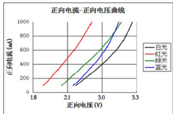
Fig 5. Forward Voltage vs. Forward Current, T_a = 25^\circ\text{C}
