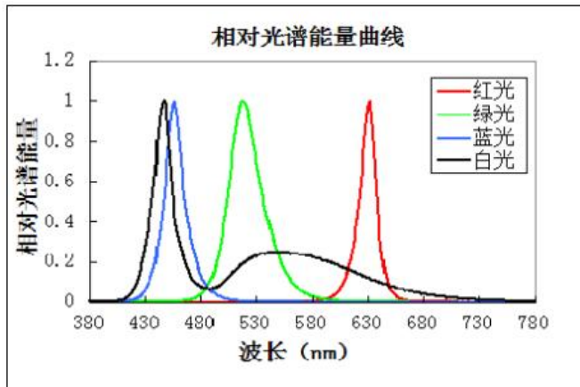
Fig 2. Color Spectrum, T_a = 25^\circ\text{C} , RH60%
