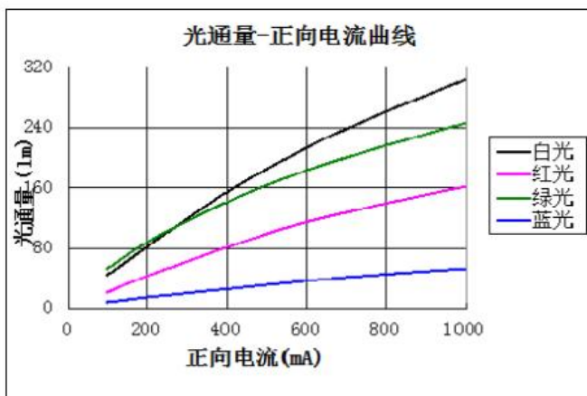
Fig 4. IF--- Luminous flux, T_a = 25^\circ\text{C}
