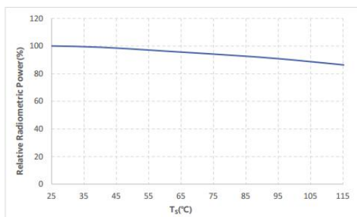
Fig 5. Relative Radiometric Power VS. Solder Temperature , IF=700mA
