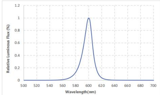
Fig 1. Relative Spectral Luminous Flux Distaibution for Dominant Wavelength 595nm, IF=700mA, Ta = 25°C, RH60%
