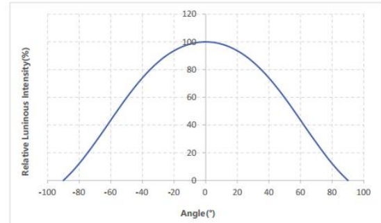
ig 2. Viewing Angle Distribution , IF=700mA, Ta = 25°C, RH60%
