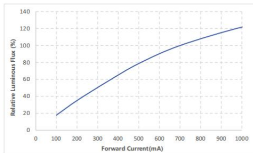
Fig 3. Relative Luminous Flux VS Forward Current, Ta = 25°C, RH60%
