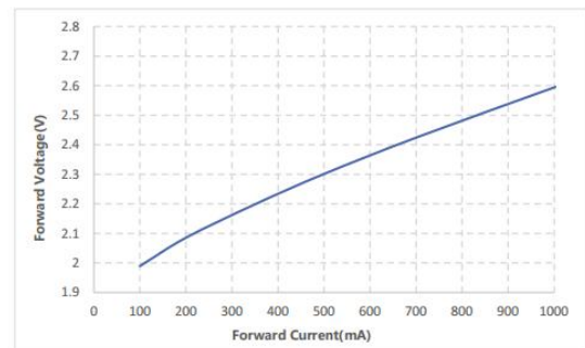
Fig 4. Forward Voltage VS. Forward Current Ta = 25°C, RH60%
