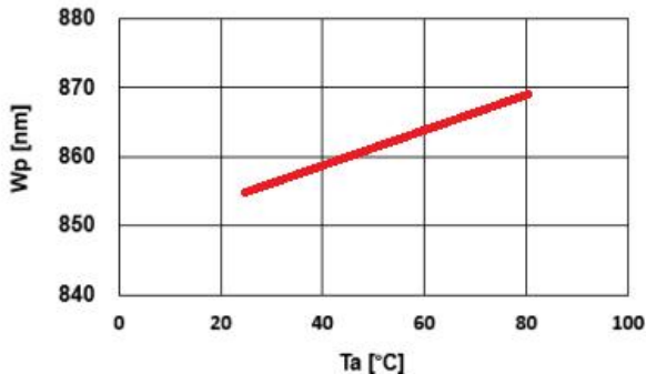
Fig.5 – Peak Wavelength (@250mA) vs. Ambient Temperature
