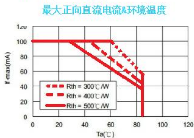
Fig.6- Maximum Driving Forward DC Current vs.Ambient Temperature (Derating based on T_j \text{ max}=115^\circ\text{C} )
