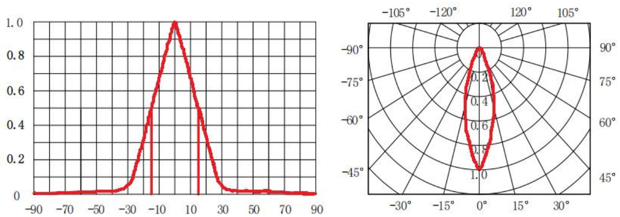
配光曲线 Light distribution curve
